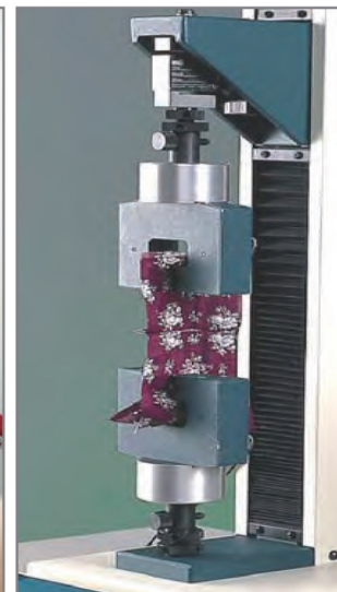
Seam slippage tests using pneumatic grips
